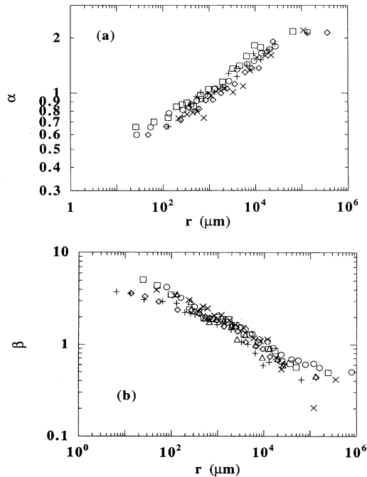
FIG. 9. Evolution of the parameters \alpha [Fig. 3(a)] and \beta [Fig. 3(b)] with the scale r , for different values of R_\lambda . \square , 1960; \circ , 4700; \circ , 1260; + , 3700; diamonds, 2100.
